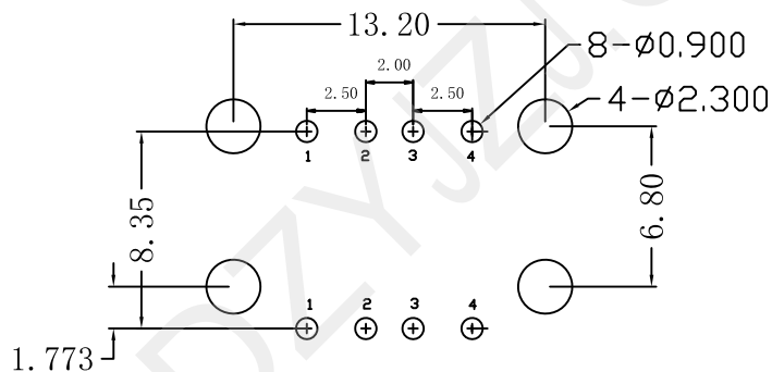
RBCOMMENDBD P.C.B PATTRN LAYOUT
